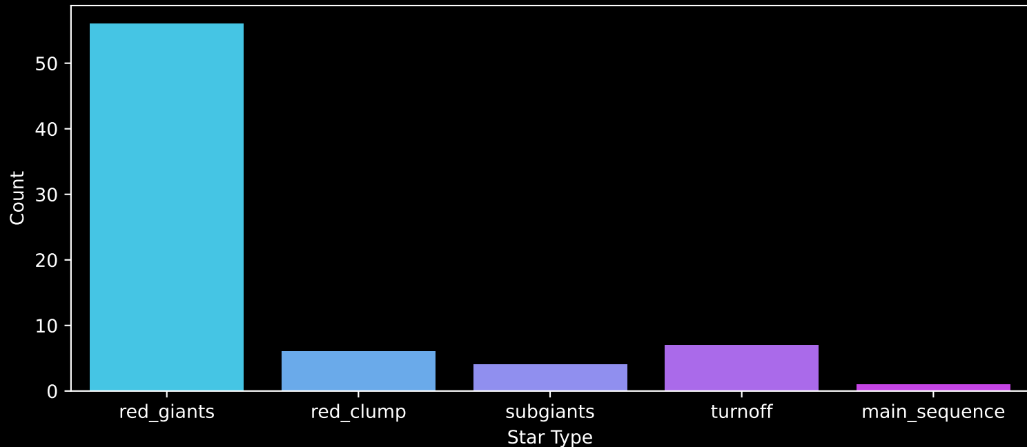
APOGEE DR17 Field: [LMC30] Count plot of Star Type
