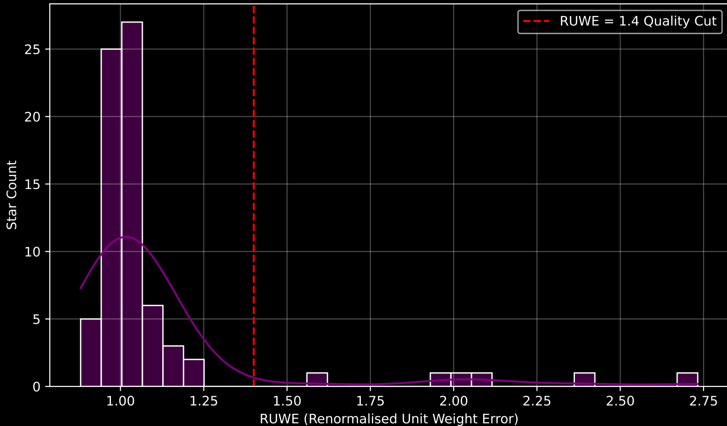
GAPOGEE DR17 Field [LMC30] RUWE Distribution (n= 74)
