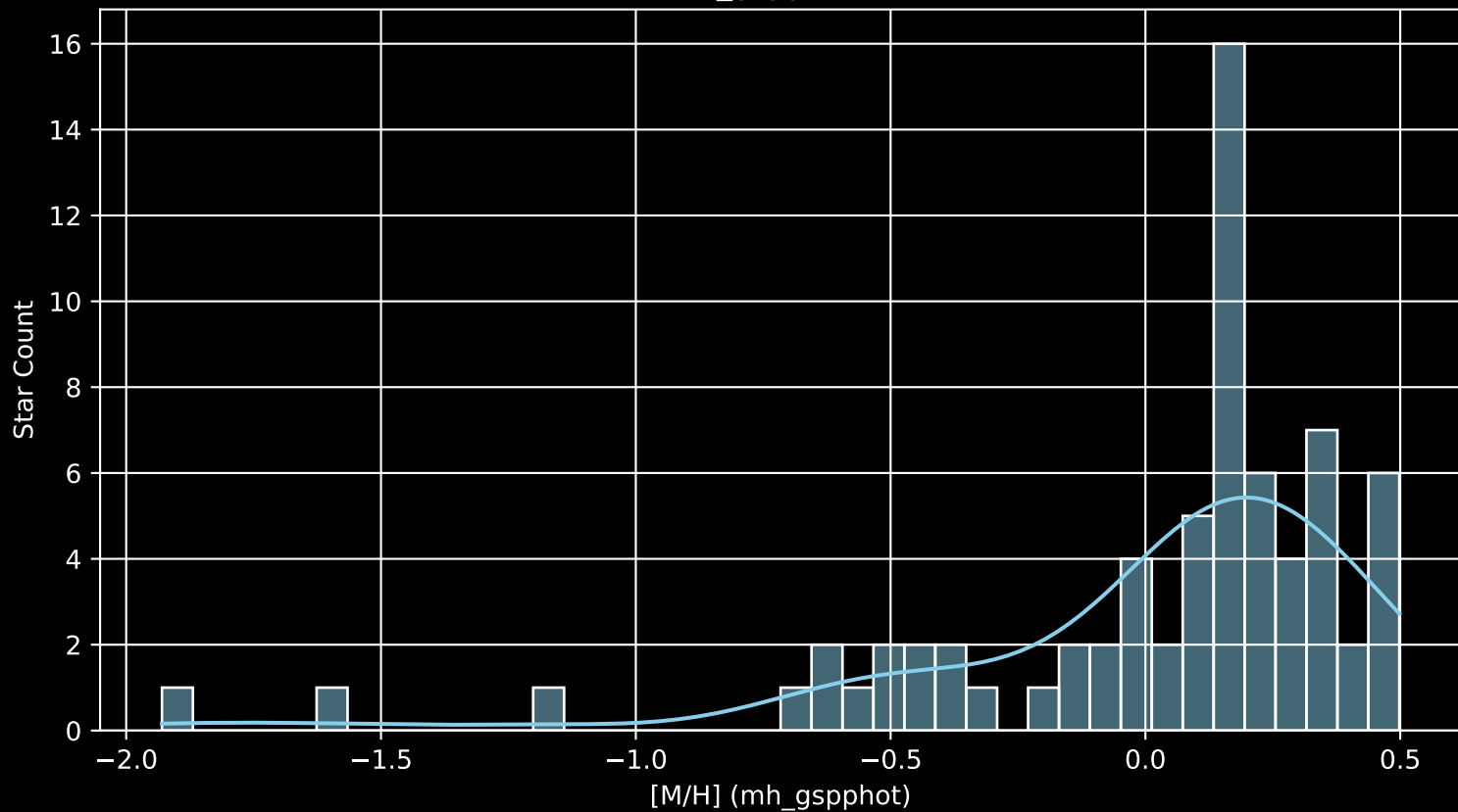
APOGEE DR17 Field: [LMC30 [M/H] (mh_gspphot) (n= 71)
