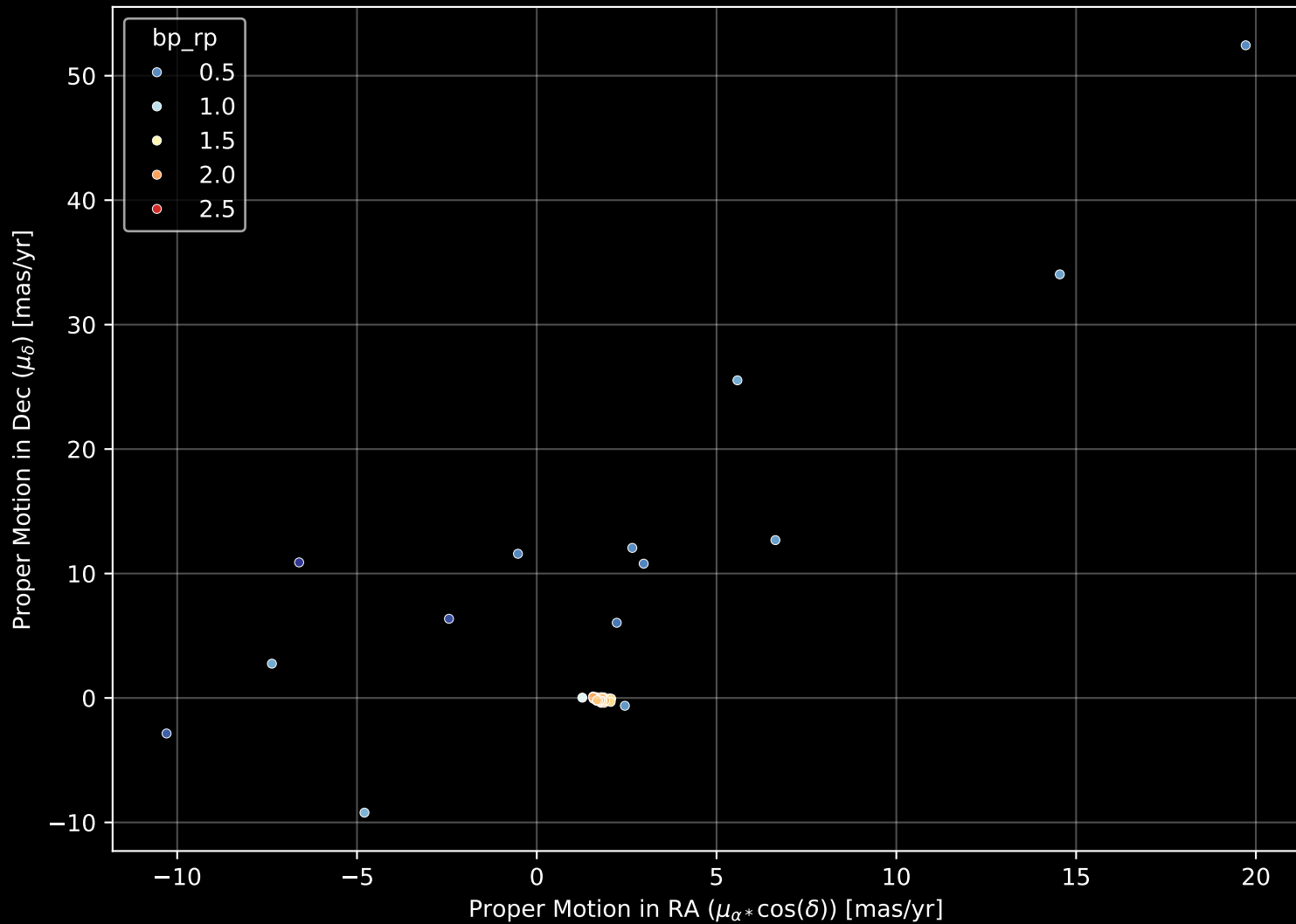
APOGEE DR17 Field: [LMC30] Proper Motion Diagram (n= 74)
