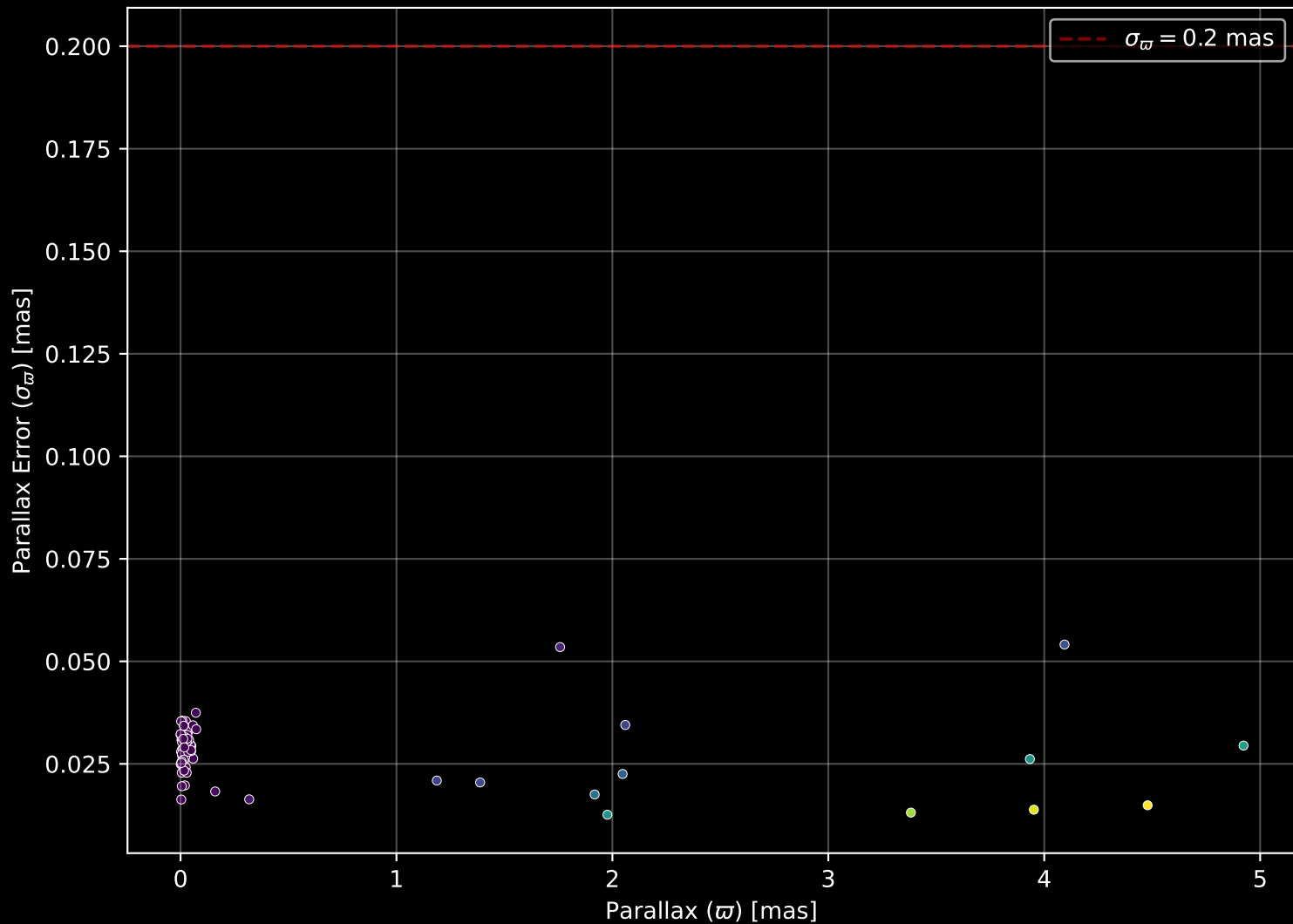
APOGEE DR17 Field: [LMC30] Parallax Quality (n= 74)
